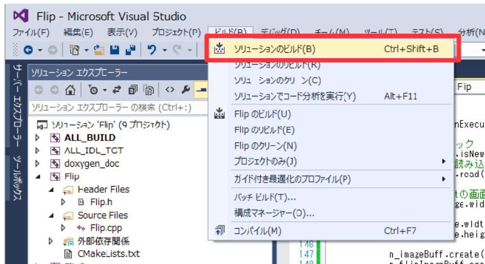
Visual Studio
