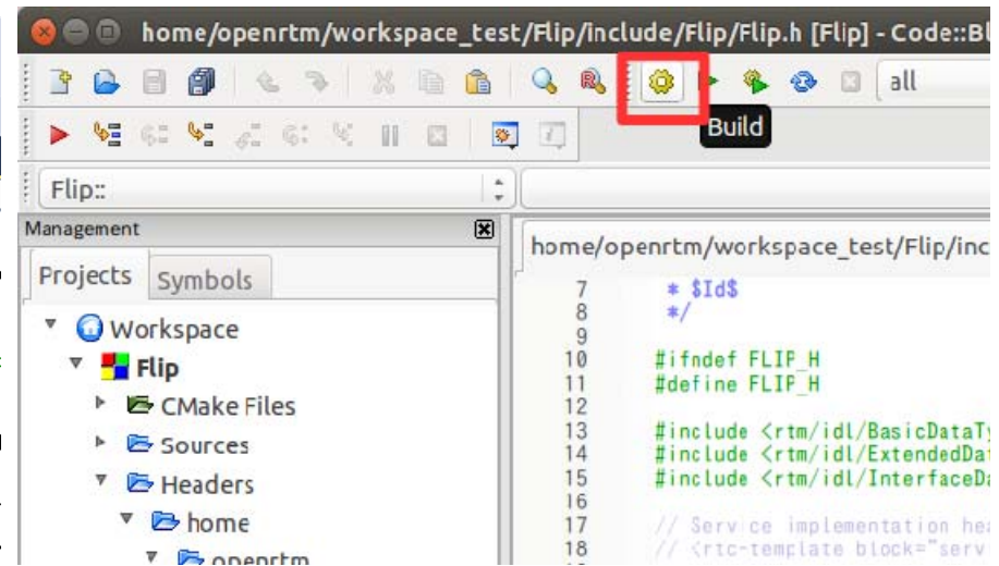
Code::Blocks
