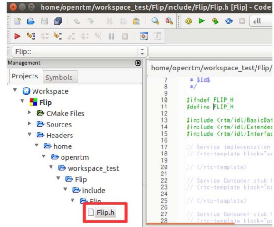
Code::Blocks
